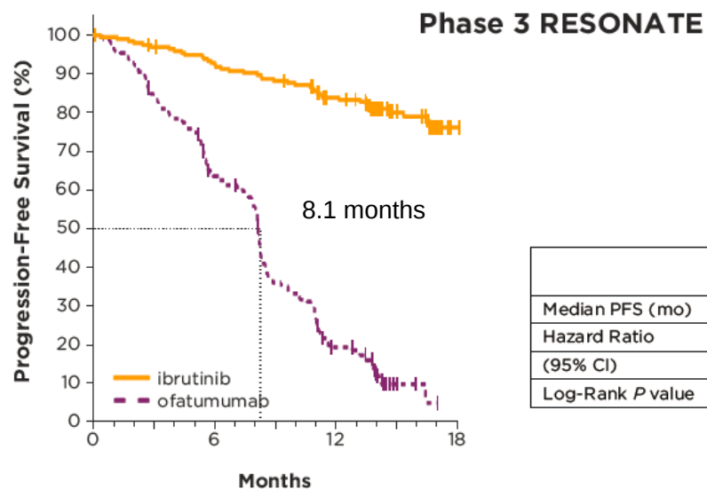
Figure 2. Progression-Free Survival
