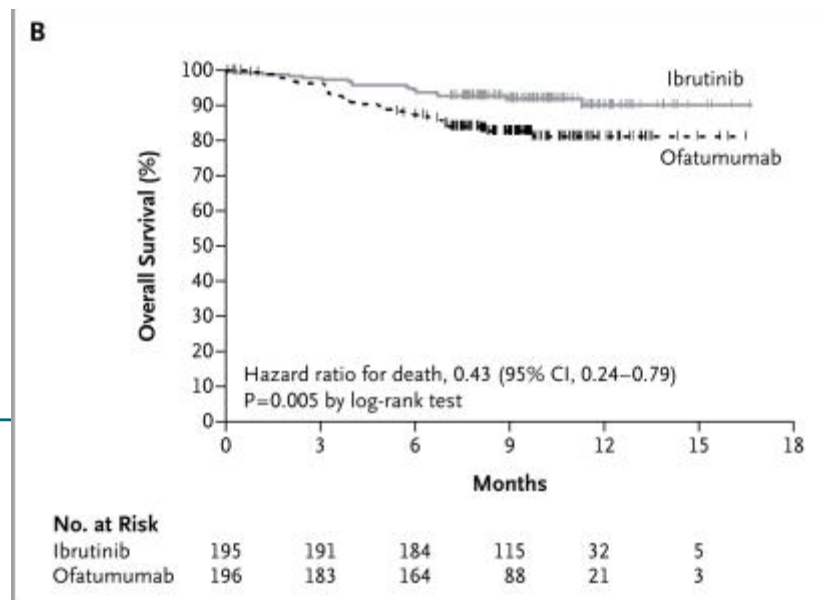
Figure 1. Overall Survival
